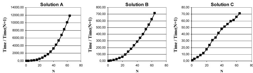
Fig. 1. Comparative time spent for running the three implement solutoins as N linearly grows.
